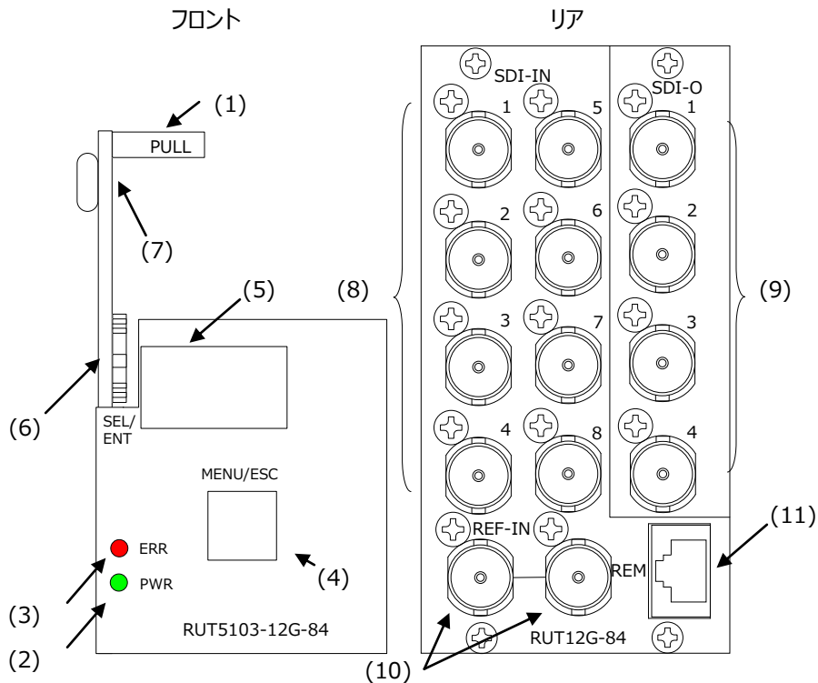
RUT5103-12G-84
