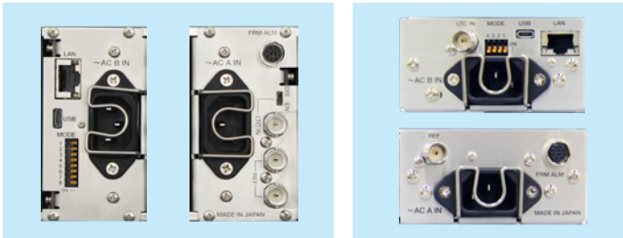
C5002 LAN, USB, REF入力, LTC入力 C5001 LAN, USB, REF入力, LTC入力
