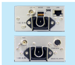
C5001 LAN, USB, REF入力, LTC入力
